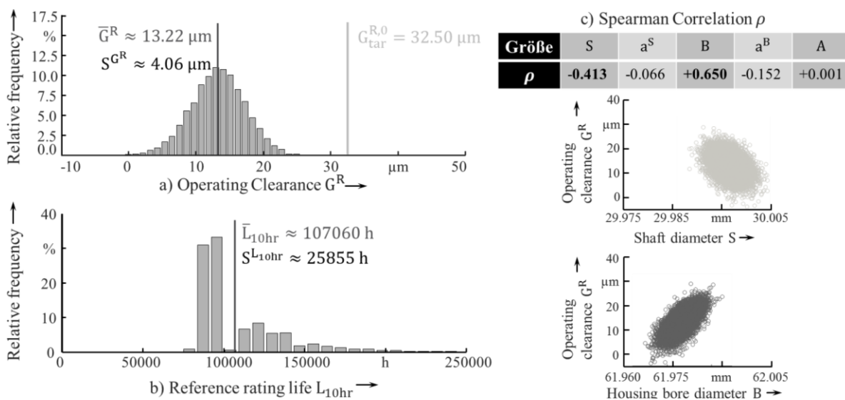
Figure 6. Results of the improved tolerance specification:
