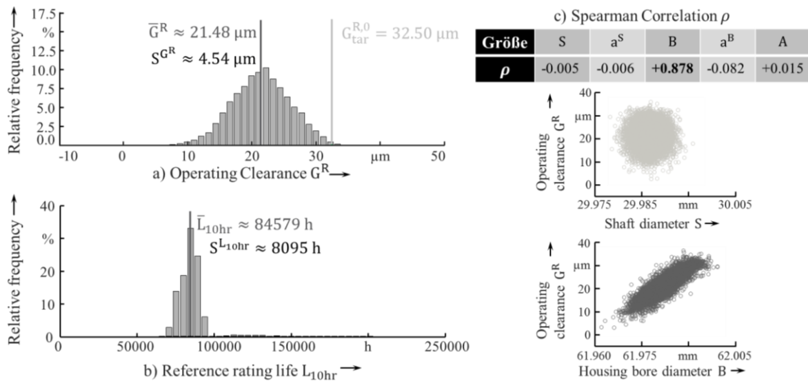
Figure 5. Results of the initial tolerance specification:
